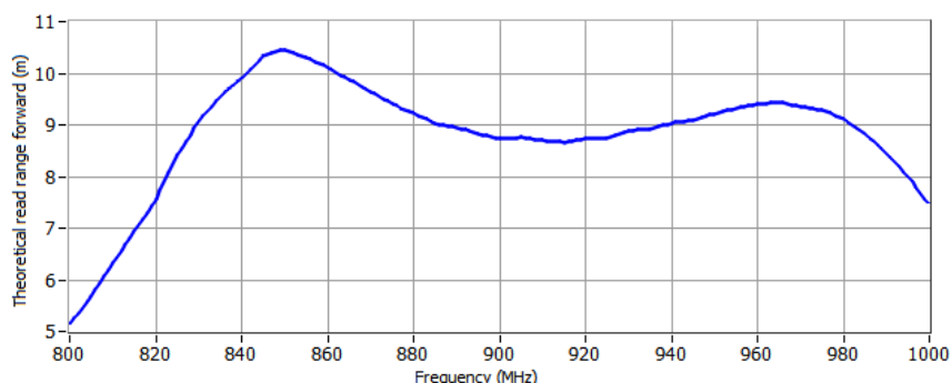
Figure 1: Read range
